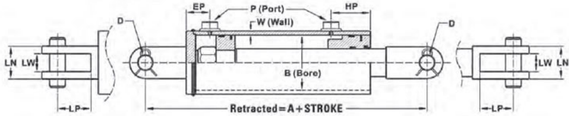
Dimensional Data (Unit: Inch)
