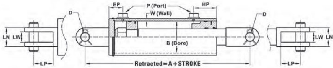
Dimensional Data (Unit: Inch)
